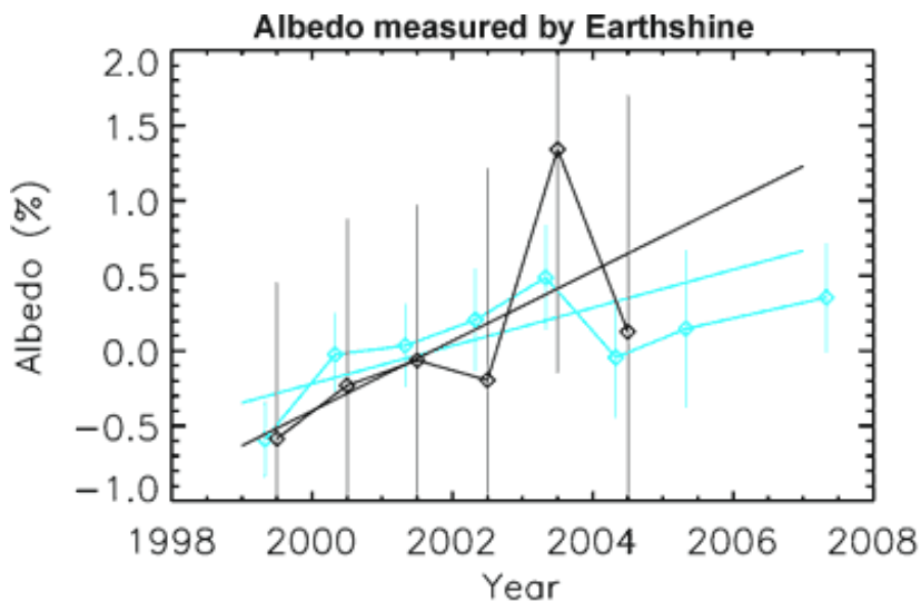
Figure 1: Earth albedo anomalies as measured by earthshine. In black are the albedo
